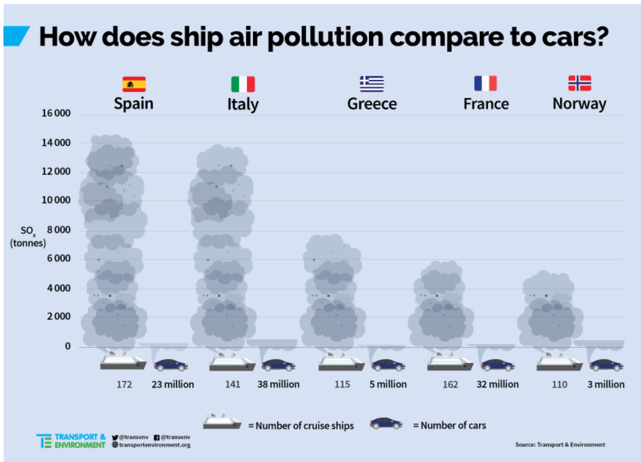
Figure 6: Comparison of SO x pollution from cruise ships in individual EEZs and domestic car fleet in each corresponding country.
